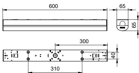
CoreLine Batten BN120C-BN126C
