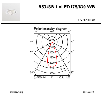
IFPC1_RS343B1xLED17S830WB
